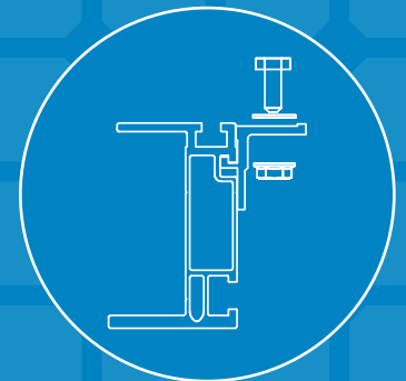
SOLARMOUNT HD RAIL W/ BOTTOM MOUNT CLIP
