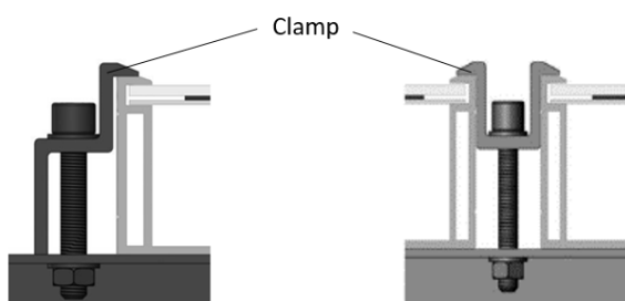
End clamp installation
