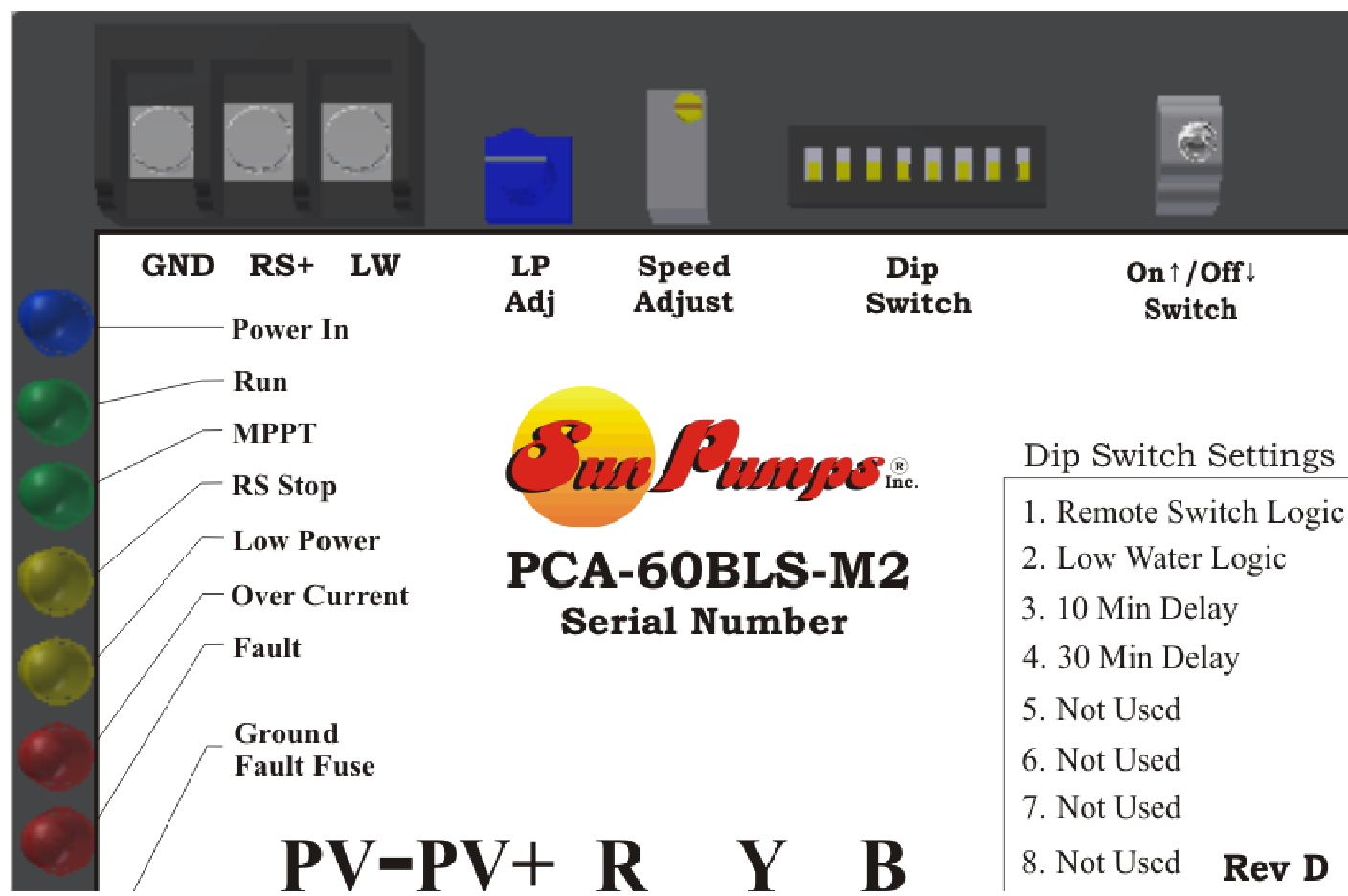
Figure 4 Dip Switch Settings
