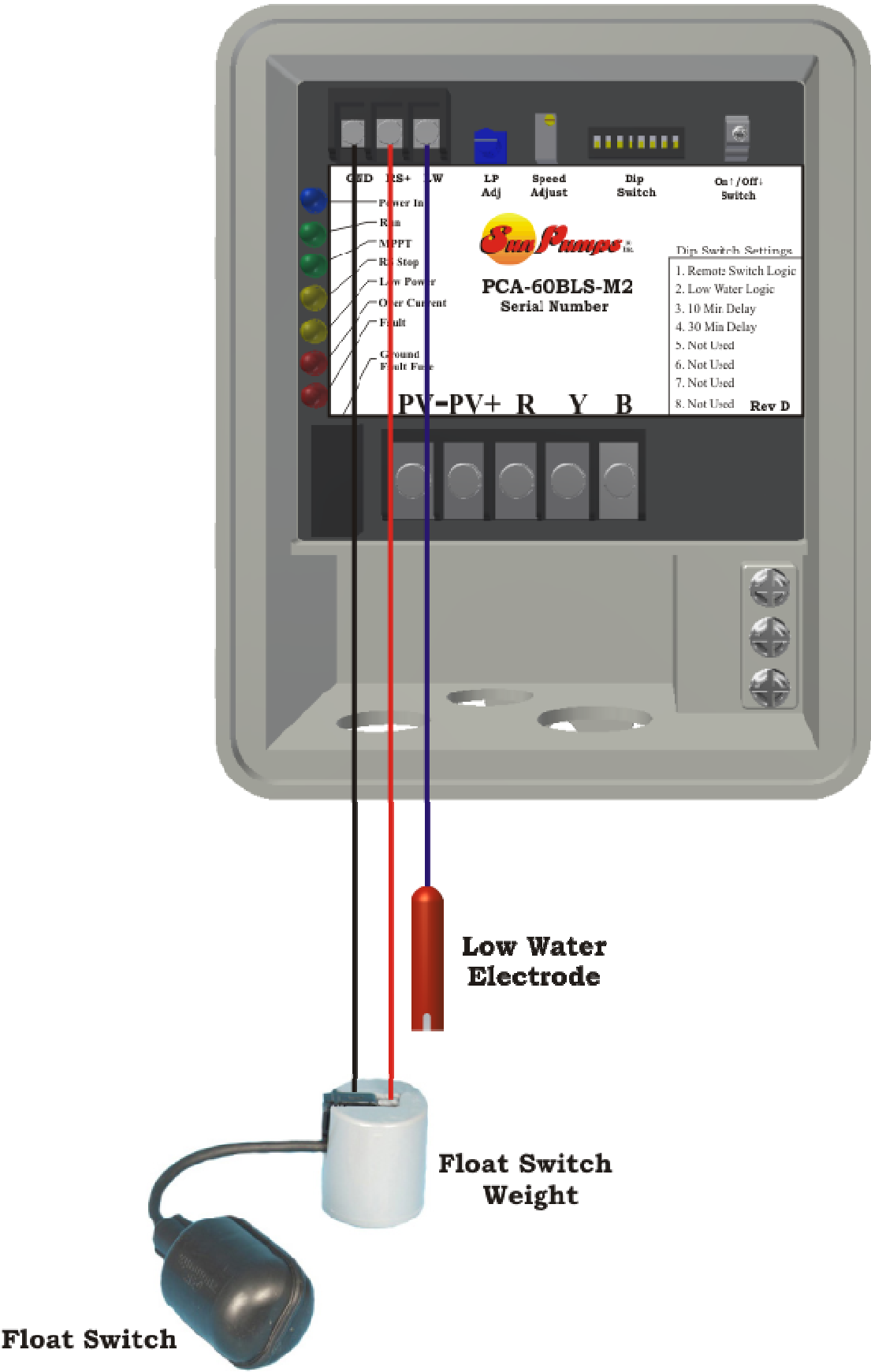
Figure 3 Controller Wiring Diagram (Auxillary)
