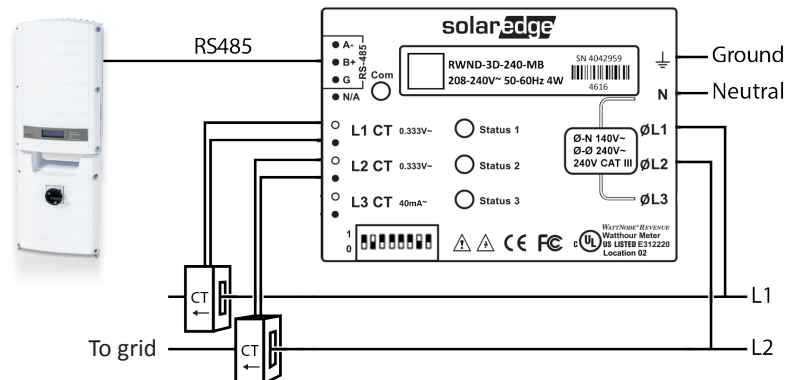
Connecting the Electricity Meter
