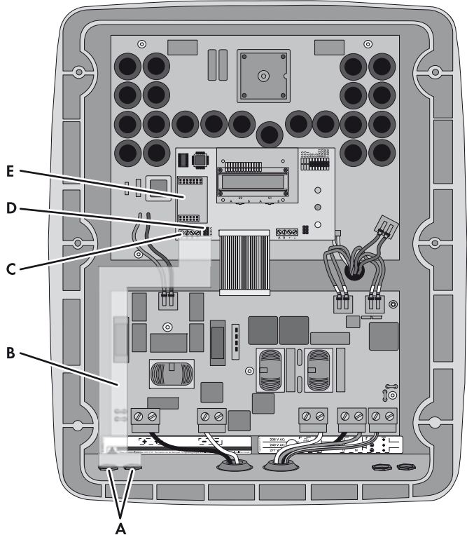
Figure 9: Overview of the connection area
