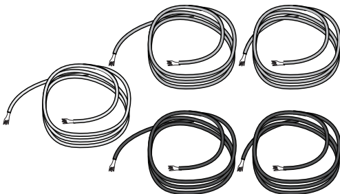
5 x #6 AWG (13.3 mm²) cables for GRID, LOAD and Neutral AC connections (labelled)
