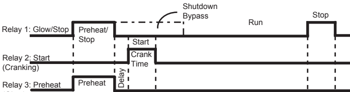
GlowStop Mode Timing Diagrams for Gen Types 1, 2, 3, 6, and 12
