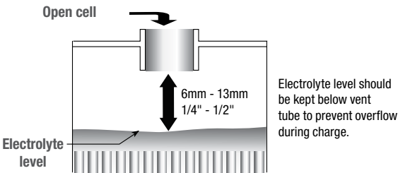
FIGURE 7: Electrolyte level
