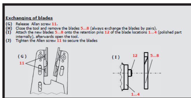
Change Blades
