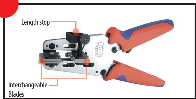
Insulation Stripper
