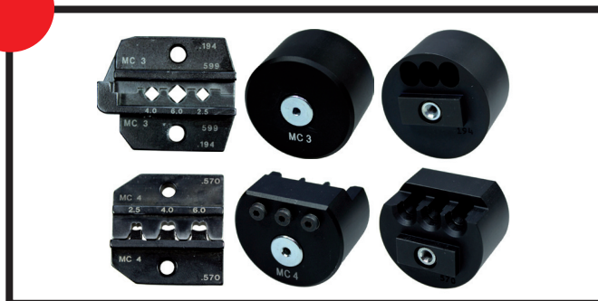
Die Sets and Locators for MC3 & MC4
