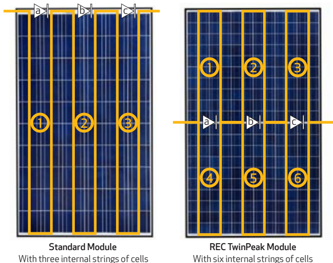
Fig. 1: Standard and REC TwinPeak modules showing representative flow of current through cell strings (1, 2, 3, 4, 5, 6) and bypass diodes (a, b, c)
