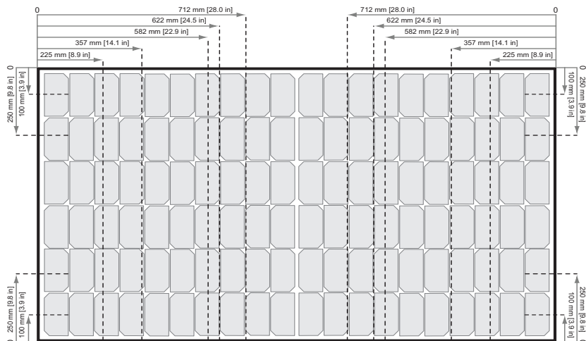
Fig. 5: Clamping of REC TwinPeak 4 Series panels using a short support
