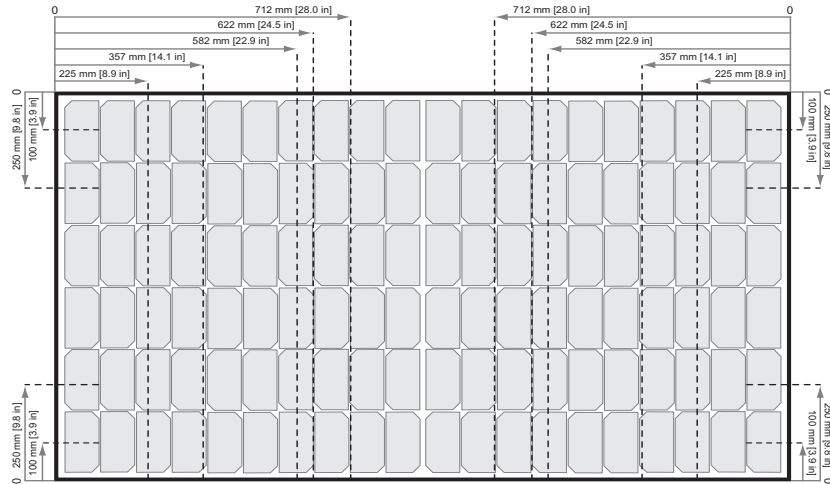
Fig. 11: Clamping of REC N-Peak 2 Series panels using a short support
