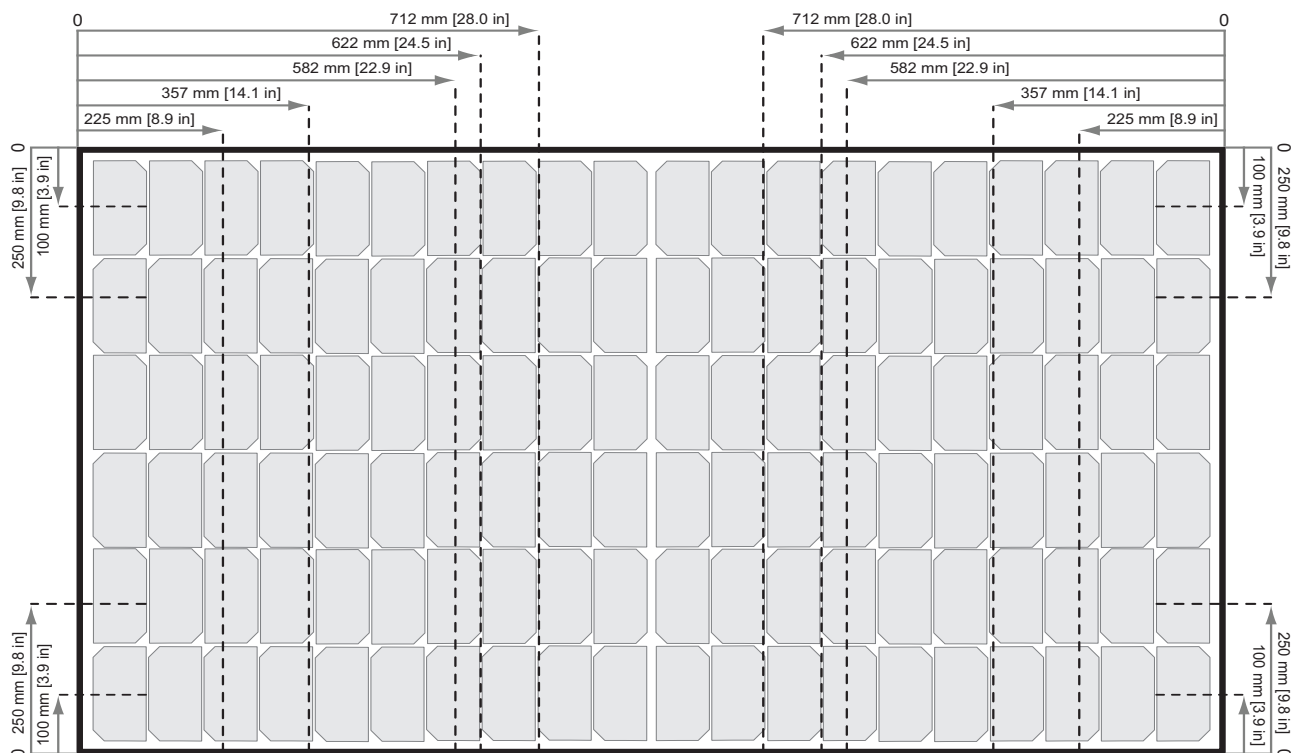
Fig. 3: Clamping of REC TwinPeak 4 Series panels with rails parallel to short side of the panel
