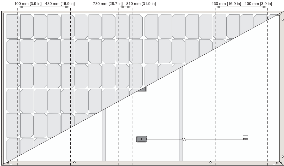
Fig. 21: Six-point mounting configuration clamping zones
