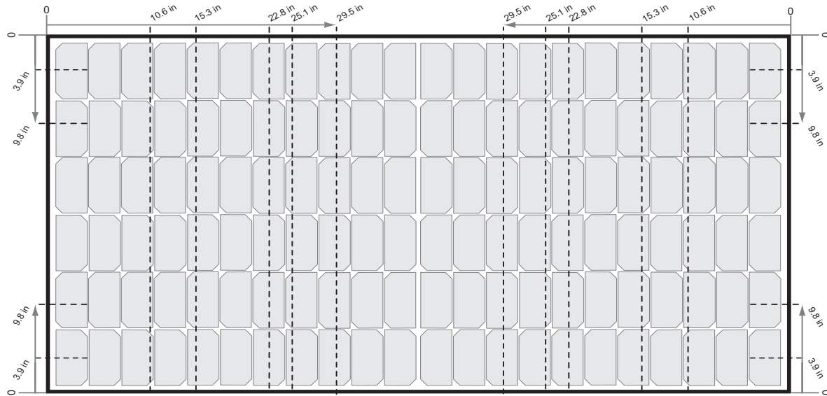
Fig. 8: Clamping of REC N-Peak 3 Black Series panels using short rails
