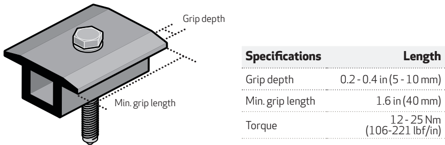
Fig. 1: Clamp specifications
