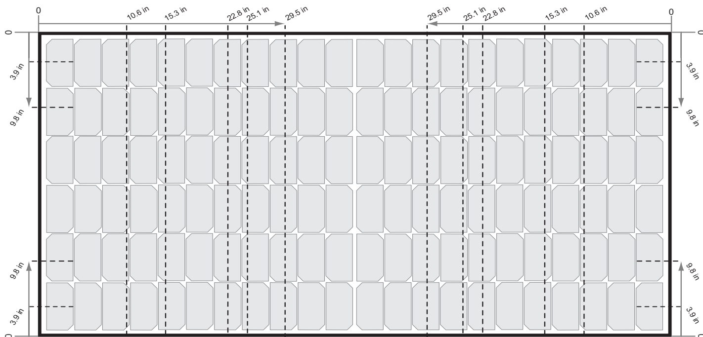
Fig. 6: Clamping of REC N-Peak 3 Black Series panels with rails parallel to short side of the panel
