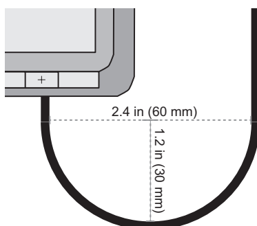
Fig. 17: Minimum cable bend radius
