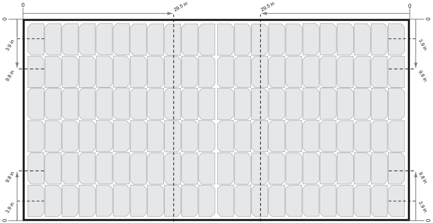
Fig. 7: Clamping of REC N-Peak 3 Black Series panels with rails parallel to long side of the panel
