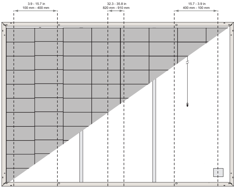
Fig. 4-2 Six-point mounting configuration clamping zones: REC Alpha Pure-RX
