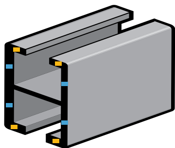
Fig. 1: Example of rail cross-section
