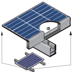
Fig. 9: Mounting hole installation: REC Peak Energy 72 Series
