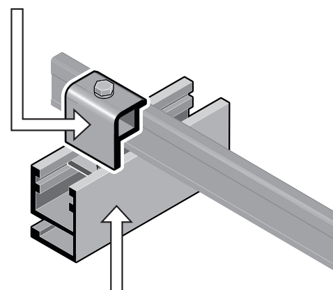
Fig. 5: Clamping the frame to rail
