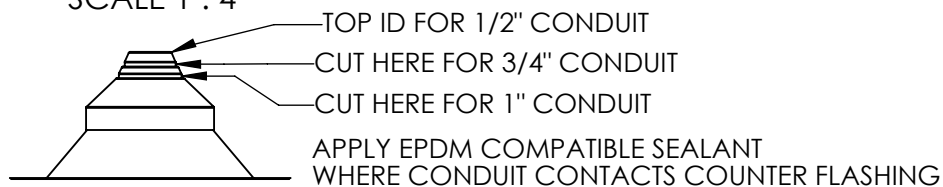
DETAIL B SCALE 1 : 4
