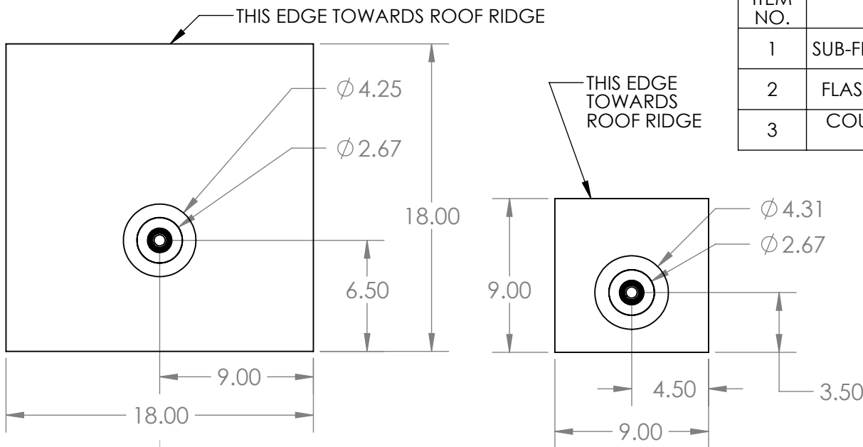
SUB FLASHING ITEM 1
