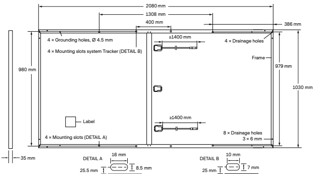
Fig. 2: External dimensions (in mm) and components for Q.PEAK DUO L-G8.1 and Q.PEAK DUO L-G8.2
