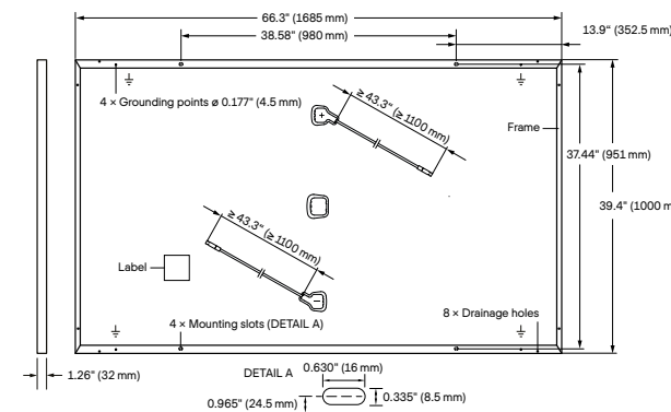
Fig. 1: External dimensions (in inch (mm)) and components for Q.PEAK DUO-G7, Q.PEAK DUO BLK-G7, Q.PEAK DUO-G7.2, Q.PEAK DUO BLK-G7.2,
