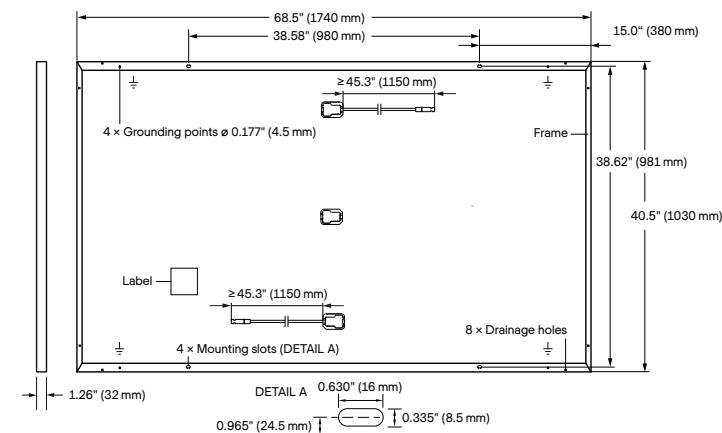
Fig. 1: External dimensions (in inch (mm)) and components for Q.PEAK DUO-G6, Q.PEAK DUO-G6+, Q.PEAK DUO BLK-G6 and Q.PEAK DUO BLK-G6+
