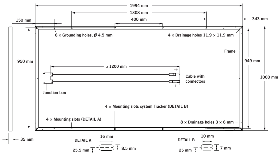
Fig. 1: External dimensions (in mm) and components for Q.PRO L-G4.1, Q.PRO L-G4.2, Q.PLUS L-G4.1, Q.PLUS L-G4.2, Q.PEAK L-G4.1, Q.PEAK L-G4.2
