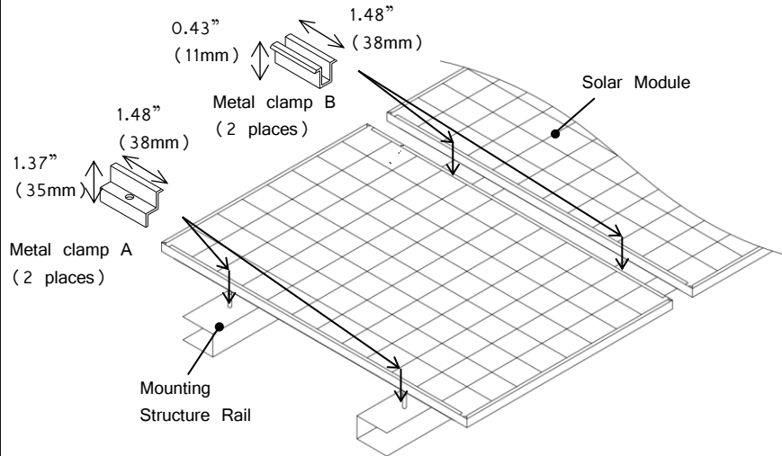
Figure 8-1 Installation A
