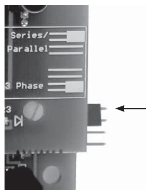
Jumper in series/ parallel location
