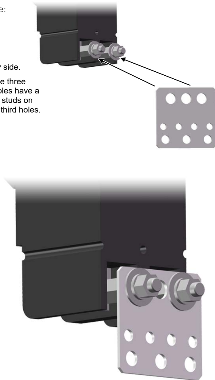
Figure 18 Assembling the DC Positive (+) Cable Plate
