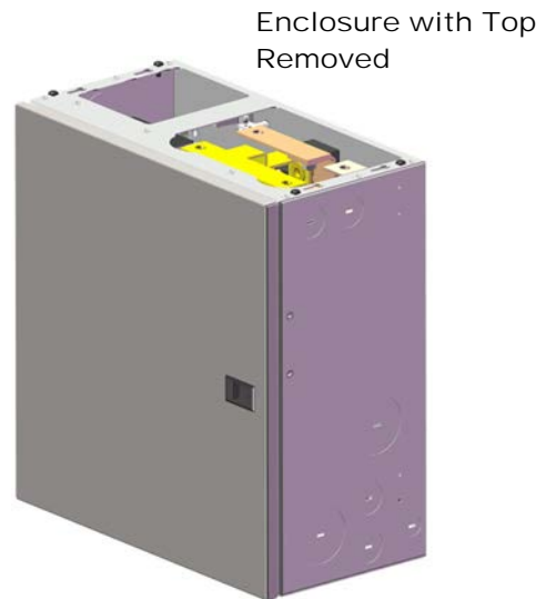
Figure 14 Removing the Top Cover from the GSLC
