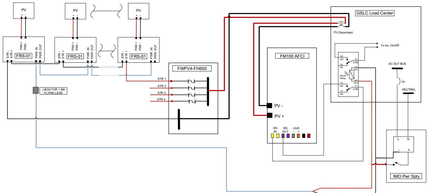
Figure 5 – Rapid Shutdown using IMO Fire Raptor MLPE devices and power supply with OutBack 24V DPDT relay
