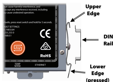
Figure 3 DIN Rail Mount
