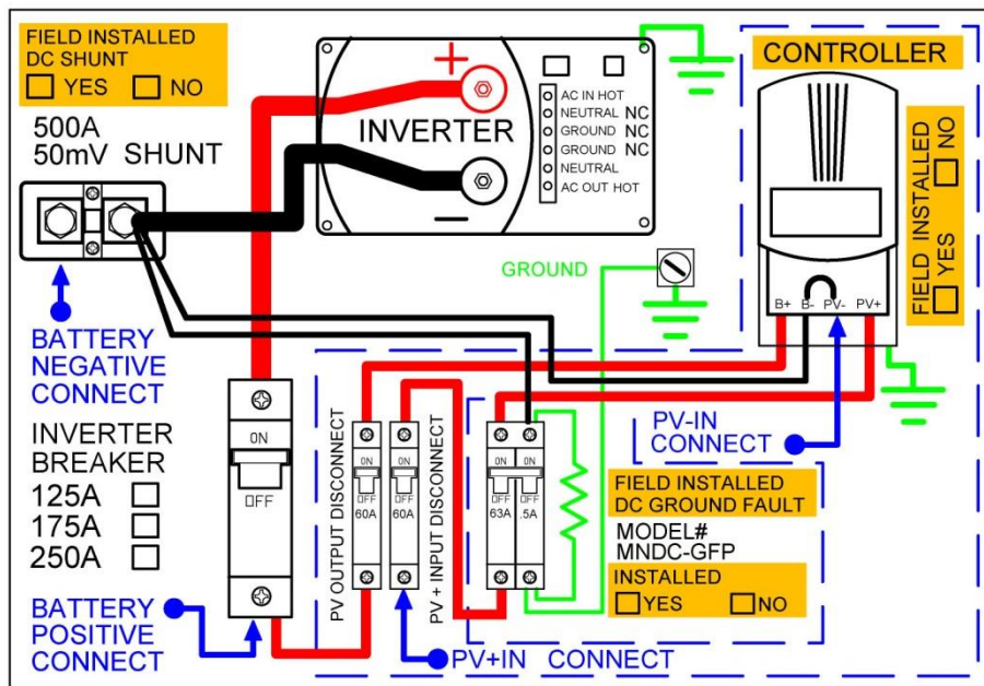
Wiring diagram
