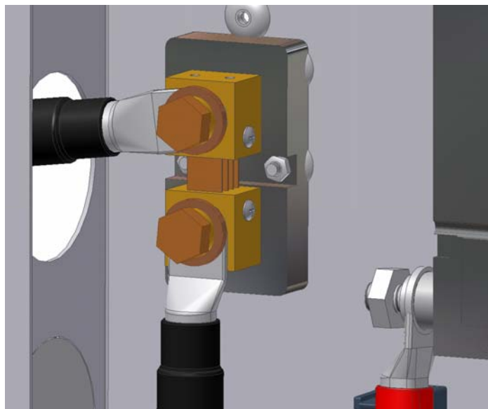
Shunt mounted vertical on bottom dimples
