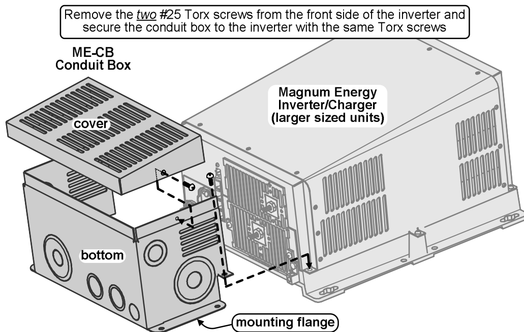
Figure 3, ME-CB Installation
