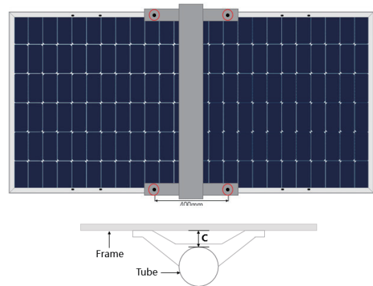
Installation with bolts into 400mm-span holes (distance between frame and tube C \geq 55\text{mm} )
