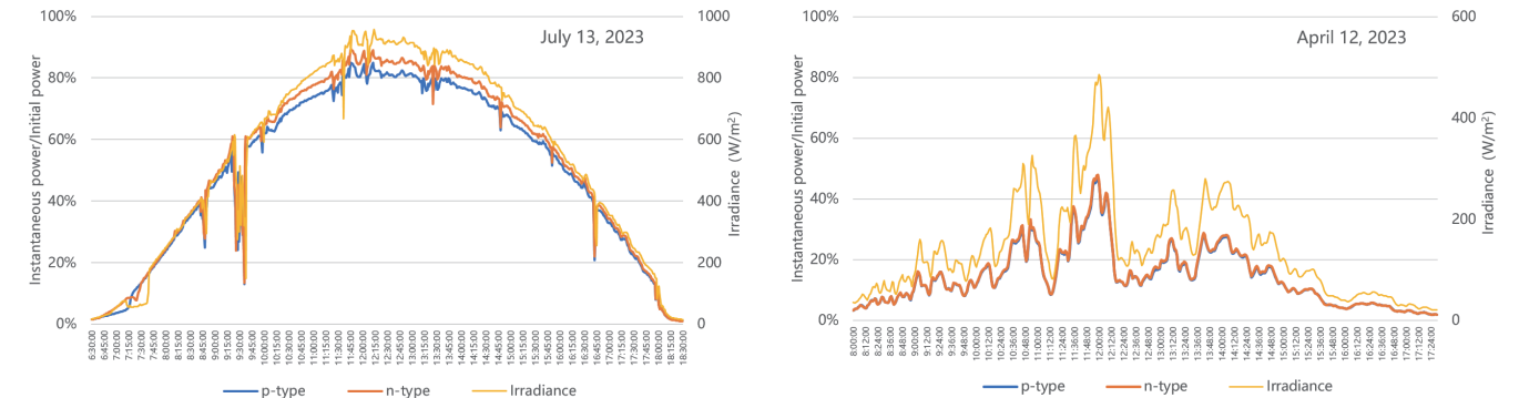
Figure 10: Power energy yield gain data of n-type modules under different irradiance in Hainan field test project
