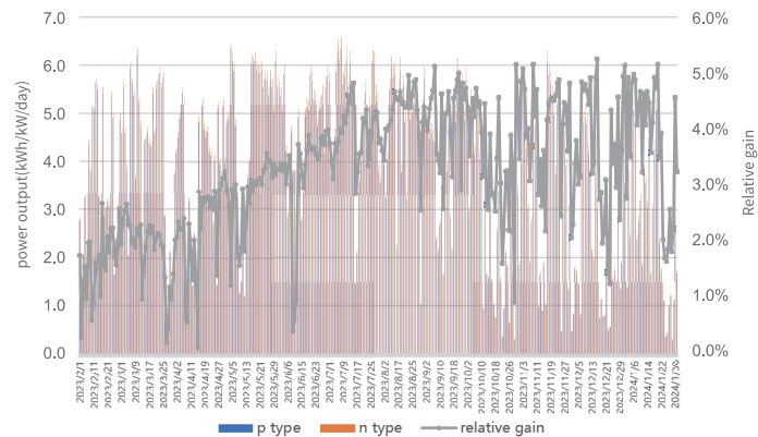
Figure 9 : Data compared between n-type module and p-type PERC module in Hainan base
