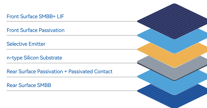
Figure 3 : Bycium+ cell structure diagram
