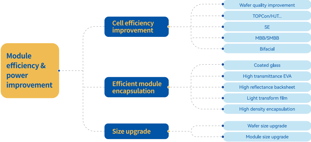
Figure 1 : The main efficiency and power improvement path of PV modules
