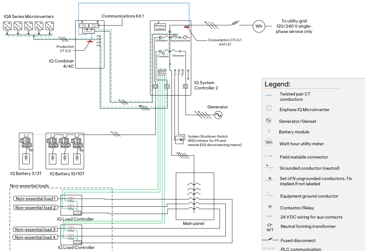
Figure 34: Whole home backup configuration with IQ8 Series Microinverters and IQ Battery 3/3T/10/10T
