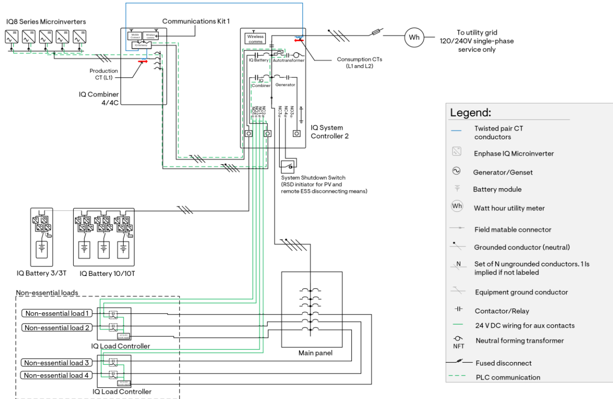
Figure 28: Whole home backup configuration using IQ8 Series Microinverters and IQ Battery 3/3T/10/10T
