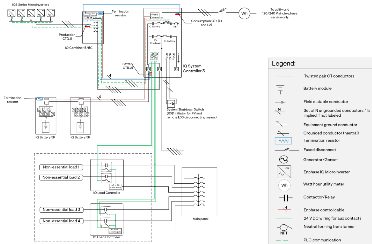
Figure 24: Whole home backup configuration with IQ8 Series Microinverters and IQ Battery 5P
