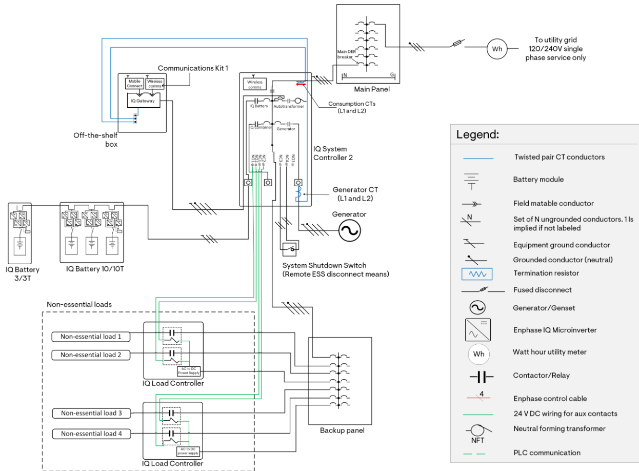
Figure 23: Battery Only grid-forming partial home backup configuration with IQ Battery 3/3T/10/10T and IQ System Controller 2
