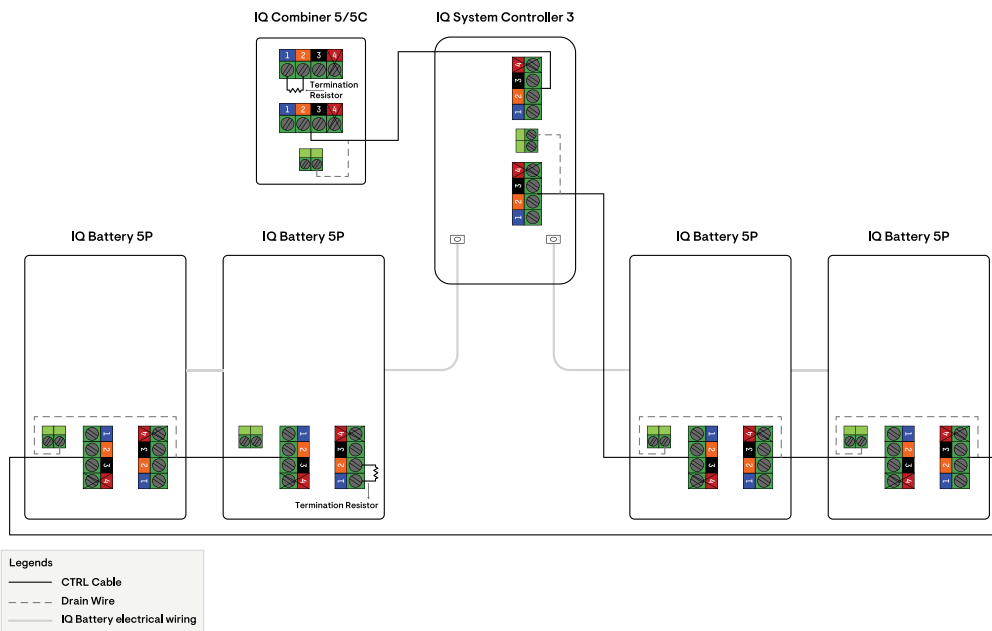
Figure 52: Control wiring sequence 2: IQ Combiner 5/5C → IQ Battery(s) 5P → IQ System Controller 3/3G
