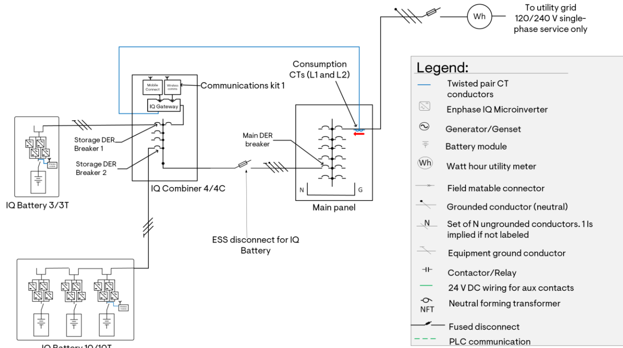
Figure 6: Battery Only grid-tied configuration with IQ Battery 3/3T/10/10T and IQ Combiner 4/4C
