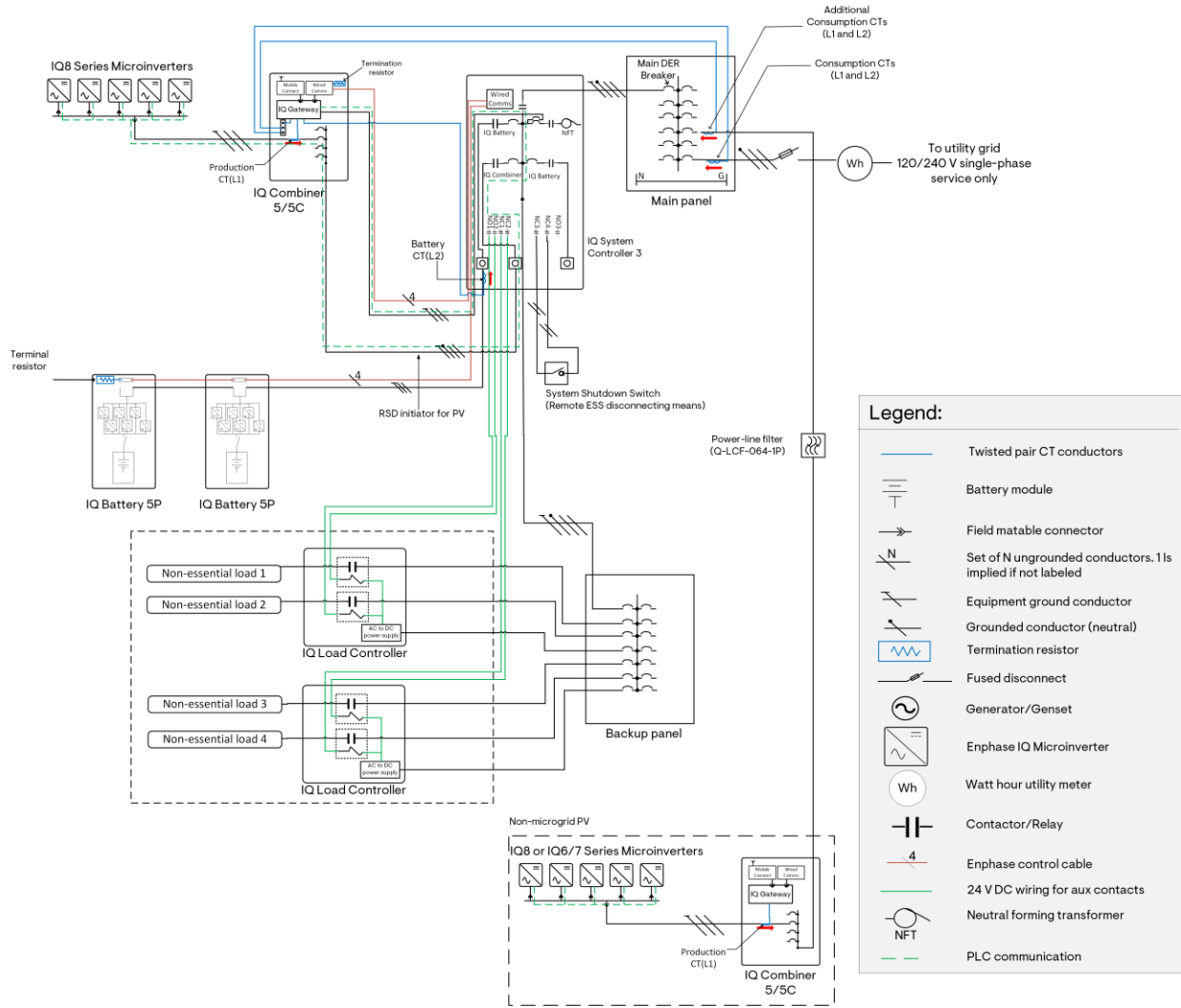
Figure 60: "Split" IQ8 PV system with an additional set of Consumption CTs
