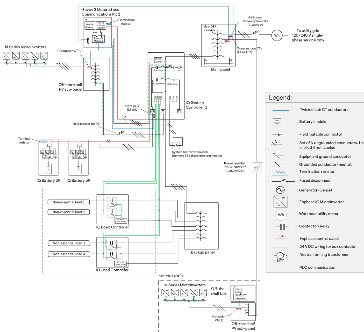
Figure 62: “Split” M Series PV system with an additional set of Consumption CTs
