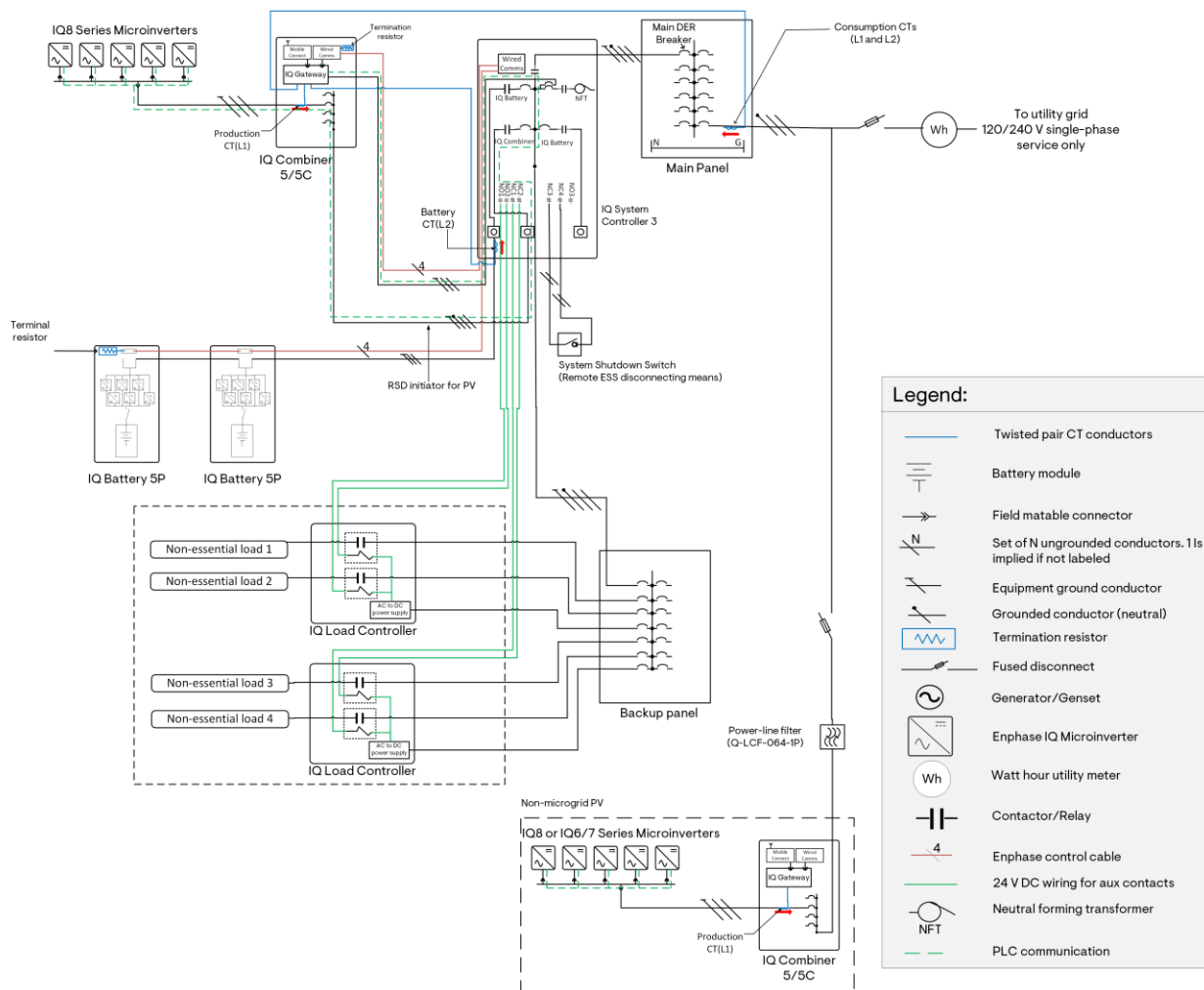
Figure 63: "Split" IQ6/IQ7 Series PV system without an additional set of Consumption CTs
