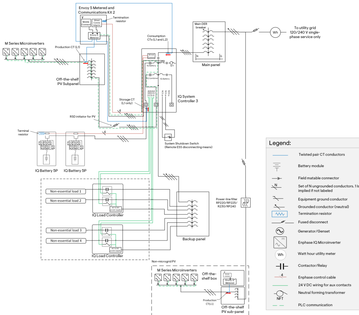
Figure 68: IQ8 Series “split” PV system without an additional set of Consumption CTs - Configuration to prevent the battery from discharging to serve loads on the main panel
