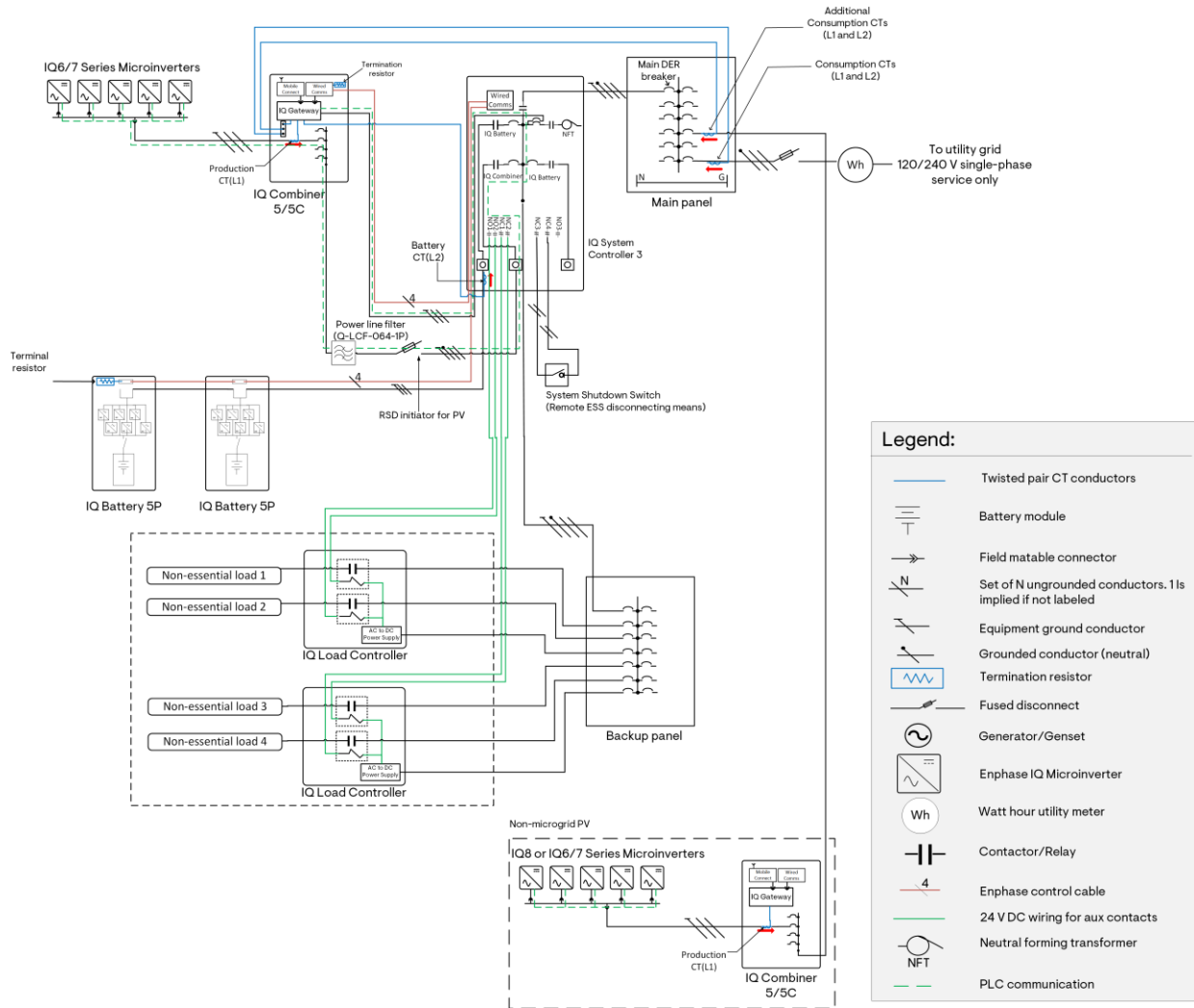
Figure 61: "Split" IQ6/IQ7 PV system with an additional set of Consumption CTs
