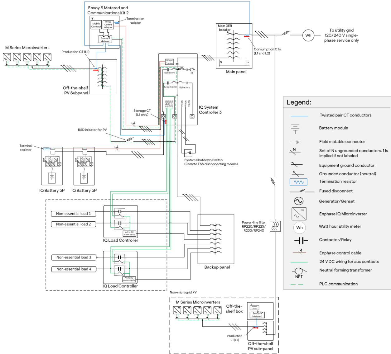
Figure 65: "Split" IQ8 Series PV system without an additional set of Consumption CTs
