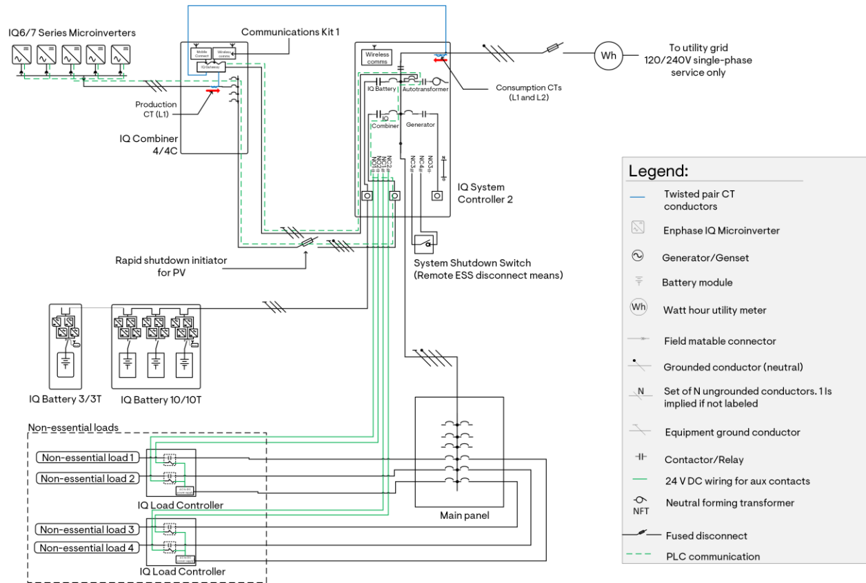
Figure 29: Whole home backup configuration using IQ6/7 Series Microinverters and IQ Battery 3/3T/10/10T
