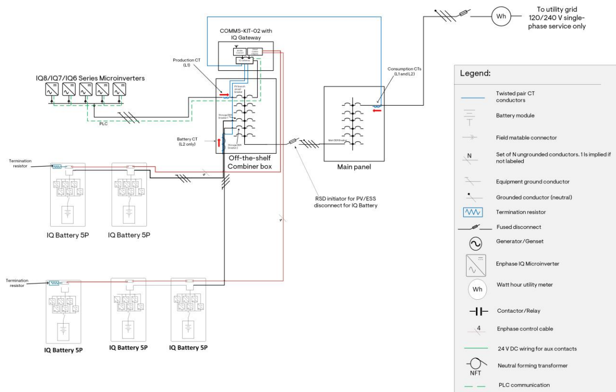
Figure 56: Solar + Battery grid-tied configuration with IQ8/IQ7/IQ6 Microinverters, IQ Battery 5P, Enphase COMMS-KIT-02, Mobile Connect cell modem and off-the-shelf combiner box
