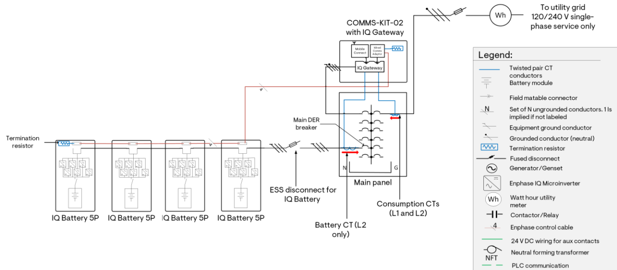
Figure 5: Battery Only grid-tied configuration IQ Battery 5P, COMMS-KIT-02, and IQ Gateway
