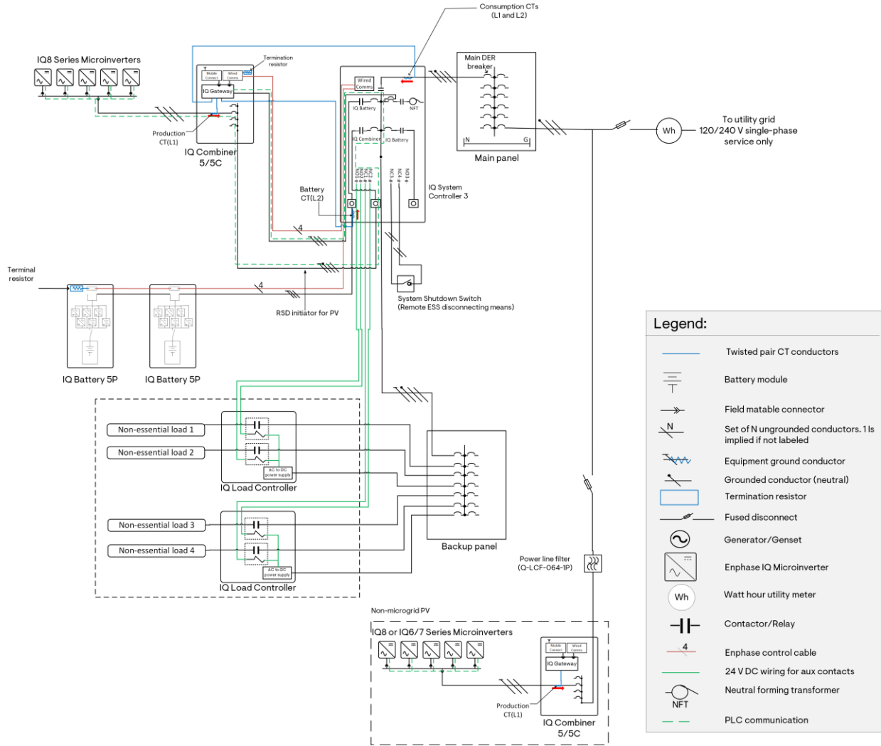
Figure 67: M Series “split” PV system without an additional set of Consumption CTs - Configuration to prevent the battery from discharging to serve loads on the main panel
