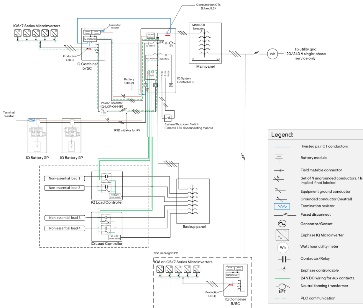
Figure 66: “Split” PV system without an additional set of Consumption CTs – Configuration to prevent the battery from discharging to serve loads on the main panel
