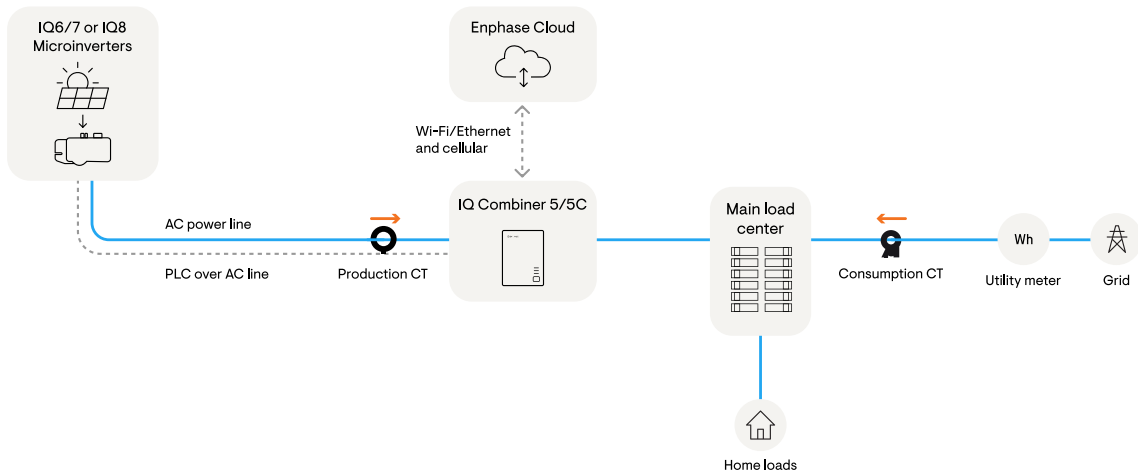
Figure 1: Consumption meters used for net grid metering
