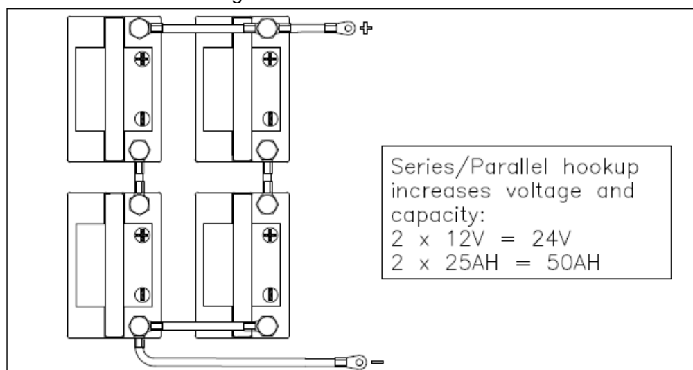
Figure 5-3. Series/Parallel Connection
