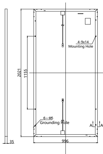
Rear View
